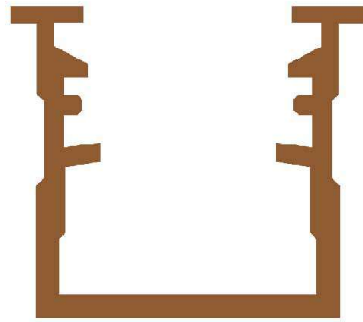
RECESSED SLIM H 10.2 mm X D 11.4 mm Profile length : 3000mm
